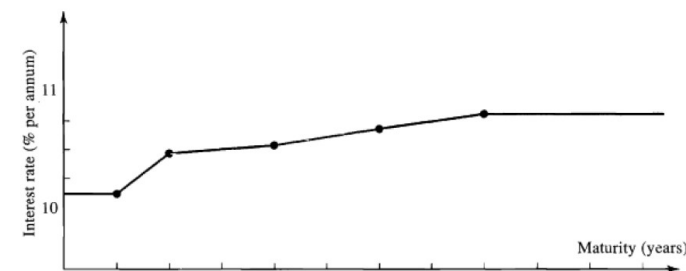
Figure 4.1 Zero rates given by the bootstrap method.
