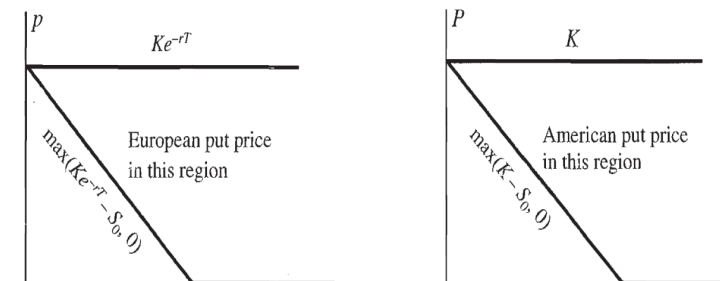
Figure 10.5 Bounds for European and American put options when there are no dividends.
