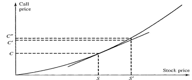
Hedging error introduced by nonlinearity.
